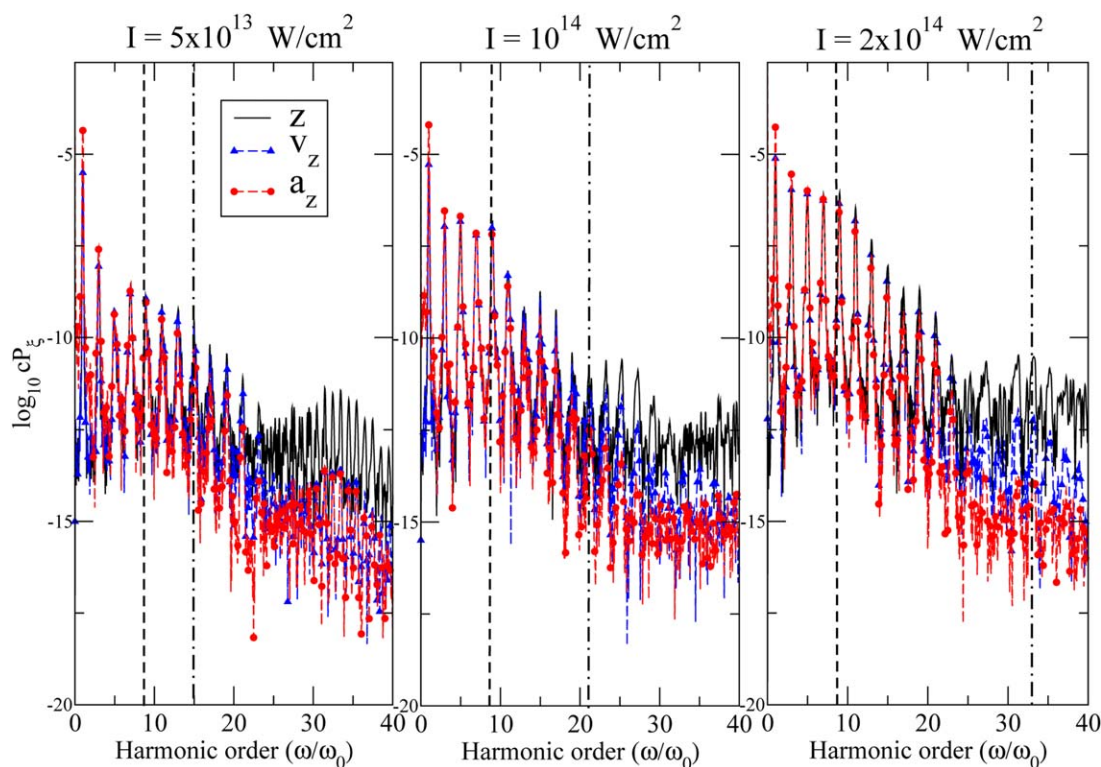
Figure 2. Velocity HHG spectra of the H atom extracted from the dipole power spectrum \omega^2 P_z(\omega) (i.e., c = \omega^2 ), the velocity power spectrum P_v(\omega) (i.e., c = 1 ), and the acceleration power spectrum P_a(\omega)/\omega^2 (i.e., c = 1/\omega^2 ) calculated with the 6-aug-cc-pVTZ basis set and laser intensities I = 5 \times 10^{13} W/cm 2 , I = 10^{14} W/cm 2 , and I = 2 \times 10^{14} W/cm 2 . The ionization threshold ( I_p/\omega_0 , vertical dashed line) and the harmonic cutoff in the three-step model N_{\text{cutoff}} (vertical dot-dashed line) are also shown.
