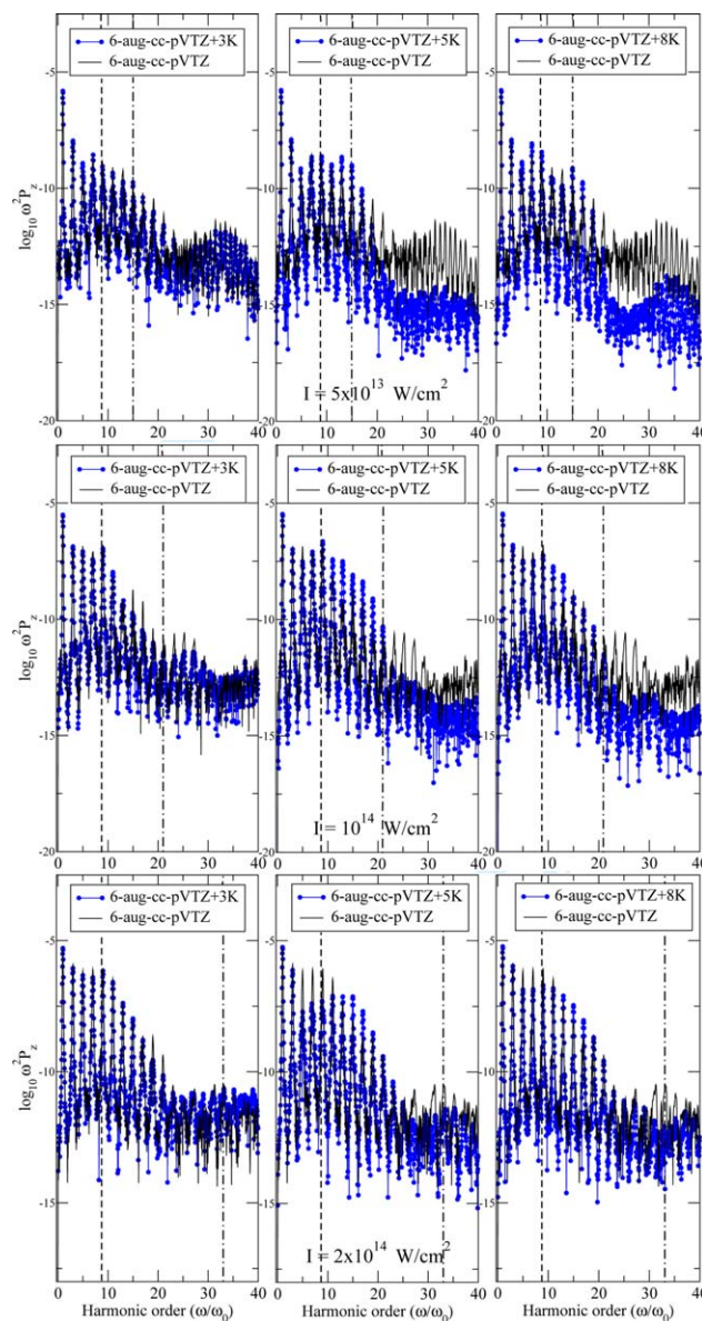
Figure 6. Comparison among the velocity HHG spectra of the H atom extracted from the dipole power spectrum \omega^2 P_z(\omega) calculated with the 6-aug-cc-pVTZ basis set plus 3 (left), 5 (middle), and 8 (right) Gaussian continuum (K) functions. The laser intensity is I = 5 \times 10^{13} W/cm 2 (top), I = 10^{14} W/cm 2 (middle), and 2 \times 10^{14} W/cm 2 (bottom). The ionization threshold ( I_p/\omega_0 , vertical dashed line) and the harmonic cutoff in the three-step model N_{\text{cutoff}} (vertical dot-dashed line) are also shown.
