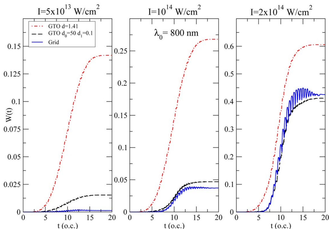
Figure 8. Ionization probability W(t) for the laser wavelength \lambda_0 = 800 and the intensities I = 5 \times 10^{13} \text{ W/cm}^2 (left), I = 10^{14} \text{ W/cm}^2 (middle), and 2 \times 10^{14} \text{ W/cm}^2 (right) obtained with the 6-aug-cc-pVTZ + 8K basis set with the original (one parameter) and modified (two parameters) lifetime models, compared with the results from the grid calculations.
