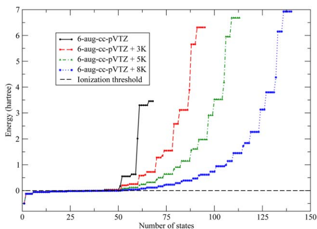
Figure 4. Distribution of the state energies obtained with the 6-aug-cc-pVTZ basis set and increasing numbers of Gaussian continuum functions ( K ).
