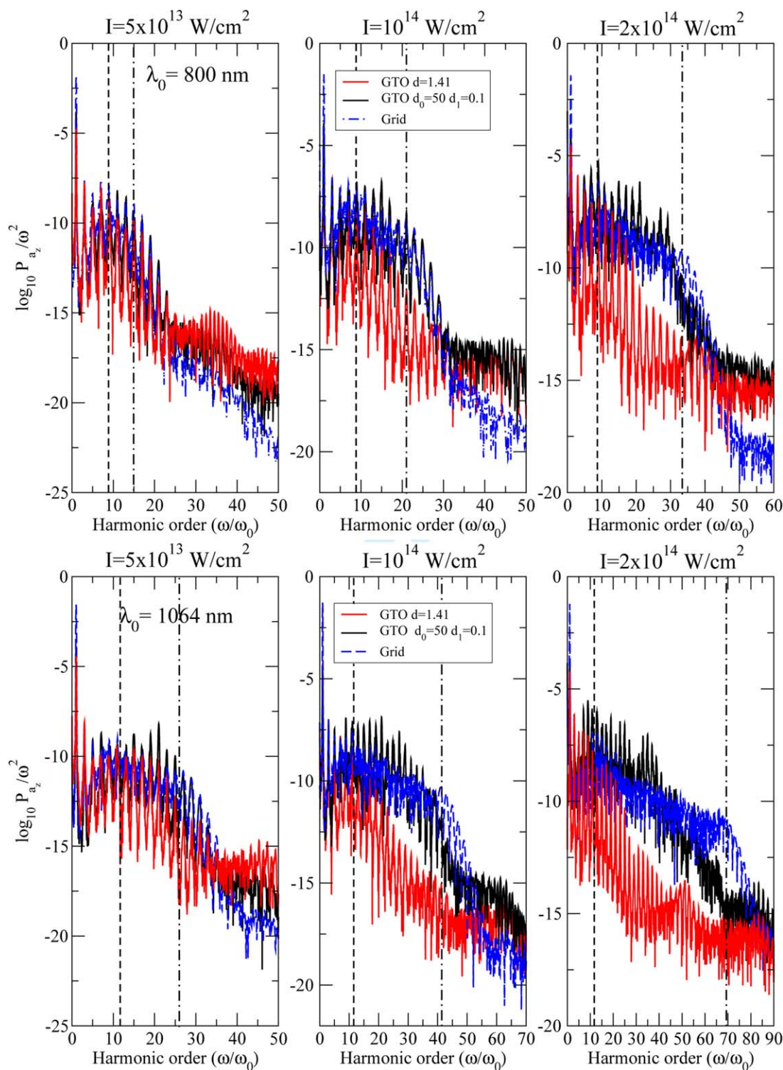
Figure 7. Velocity HHG spectrum extracted from the acceleration power spectrum P_{a_z}(\omega)/\omega^2 calculated with the 6-aug-cc-pVTZ + 8K basis set with two lifetime models and with grid calculations, for the two laser wavelength \lambda_0 = 800 nm (upper panel) and 1064 nm (lower panel), the laser intensities I = 5 \times 10^{13} , 10^{14} , and 2 \times 10^{14} W/cm 2 . The ionization threshold ( I_p/\omega_0 , vertical dashed line) and the harmonic cutoff in the three-step model N_{\text{cutoff}} (vertical dot-dashed line) are also shown.
