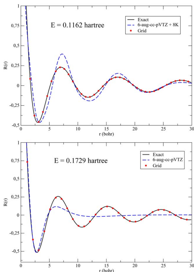
Figure 5. Comparison between the exact radial wave function R(r)^{[45]} and the radial wave function obtained using the 6-aug-cc-pVTZ + 8K basis set for a s continuum state at the energy E = 0.1162 hartree (upper panel). In the lower panel, the same comparison is done for a similar state of close energy E = 0.1729 hartree but with the 6-aug-cc-pVTZ basis set, that is, without the Kaufmann basis functions. The radial wave functions obtained in the grid calculations are also shown. Since continuum wave functions cannot be normalized in the standard way, the curves have been scaled in order to approximately have the same value at the first minimum.
