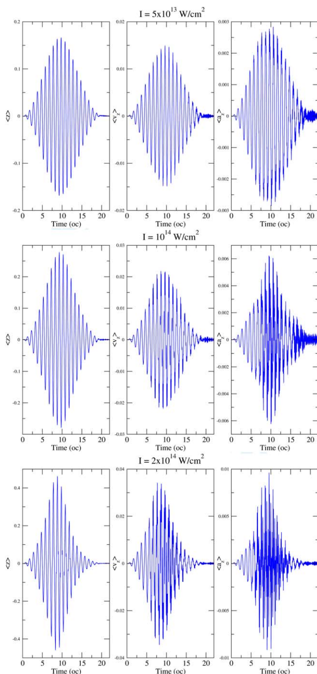
Figure 1. Time-dependent dipole z(t) (left), velocity v_z(t) (middle), and acceleration a_z(t) (right) calculated with the 6-aug-cc-pVTZ basis set for laser intensities I = 5 \times 10^{13} \text{ W/cm}^2 (top), I = 10^{14} \text{ W/cm}^2 (middle), and 2 \times 10^{14} \text{ W/cm}^2 (bottom).
