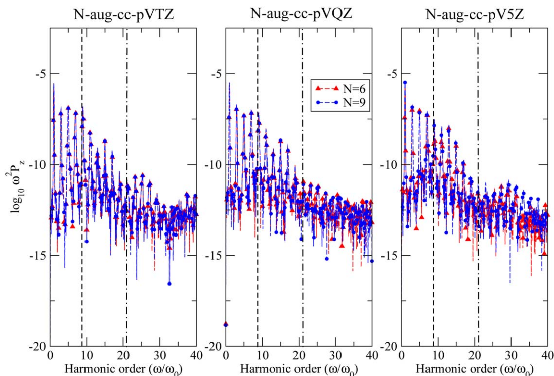
Figure 3. Velocity HHG spectrum of the H atom extracted from the dipole power spectrum \omega^2 P_z(\omega) calculated with the 6-aug-cc-pVXZ and 9-aug-cc-pVXZ basis sets with X = T (left), Q (middle) and 5 (right). The laser intensity is I = 10^{14} W/cm 2 . The ionization threshold ( I_p/\omega_0 , vertical dashed line) and the harmonic cutoff in the three-step model N_{\text{cutoff}} (vertical dot-dashed line) are also shown.
