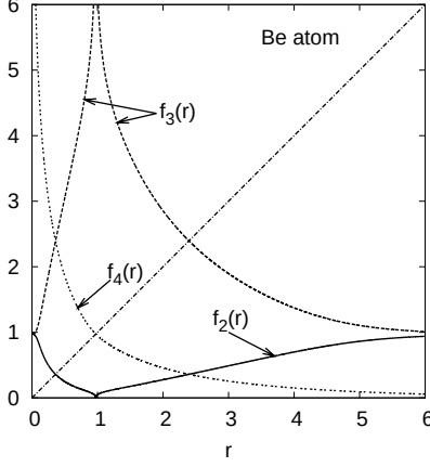
FIG. 4: The radial co-motion functions f_2(r) , f_3(r) and f_4(r) for the Be atom density. Hartree atomic units are used.
