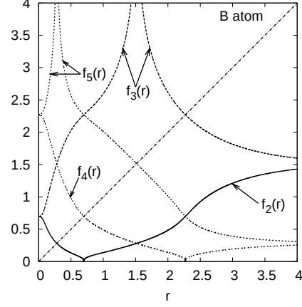
FIG. 6: The radial co-motion functions for the sphericalized B atom density. Hartree atomic units are used.
