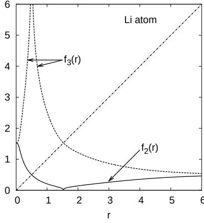
FIG. 1: The radial co-motion functions f_2(r) and f_3(r) for the Li atom density. Hartree atomic units are used.
