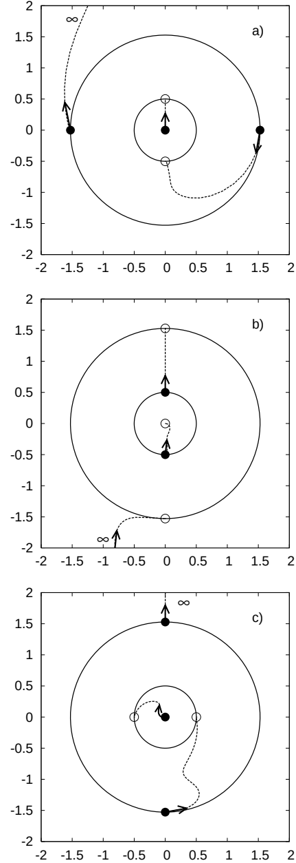
FIG. 2: The positions of the 3 electrons in the SCE state for the Li atom density. The two big circles are the projections of the spheres containing, on average in the quantum mechanical problem, 1 electron (radius a_1 ) and 2 electrons (radius a_2 ). The position r of the first electron is varied along the vertical z axis a) from 0 to a_1 , b) from a_1 to a_2 , and c) from a_2 to \infty . The other two electrons have distances from the center given, respectively, by f_2(r) and f_3(r) of Eqs. (37)-(38), and angular positions given by the minimizing angles \theta_2(r, f_2(r), f_3(r)) and \theta_3(r, f_2(r), f_3(r)) . In each panel, the starting position of the 3 electrons is represented by a full circle (●) and their final position by an empty circle (○). The dashed curves represent the “trajectories” of the 3 electrons, and the arrows their direction. The three panels are actually equivalent (see text). Distances are in atomic units.
