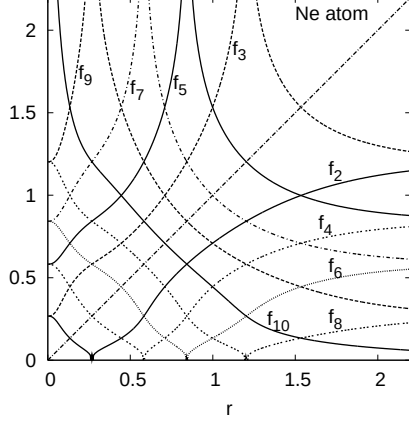
FIG. 8: The radial co-motion functions for the Ne atom density. Hartree atomic units are used.
