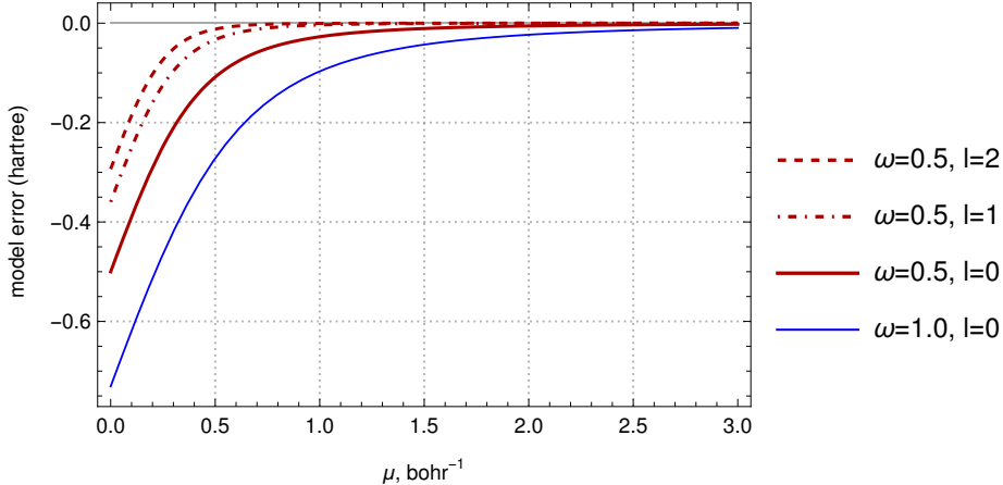
FIG. 1. Error of the energy of the model system, \Delta_0 E(\mu) , for the lowest energy state of harmonium with \omega = 1/2 (red curves), and \omega = 1 (thin blue curve), for \ell = 0 , full curves; \ell = 1 , dot-dashed curve; \ell = 2 , dashed curve.
