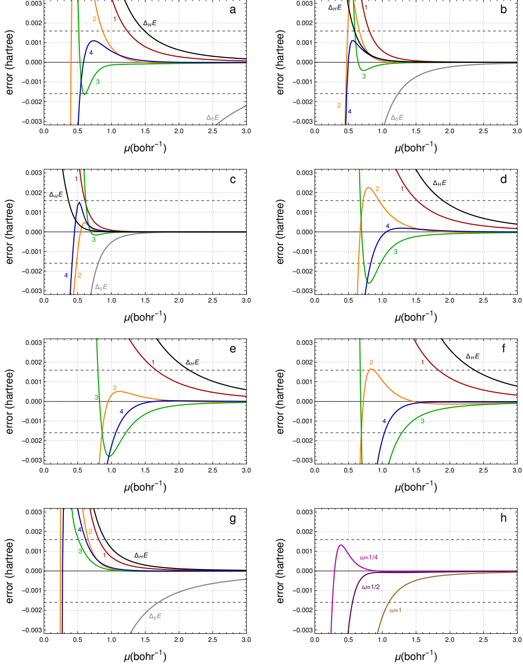
FIG. 3. Errors of the different approximations for the energy of harmonium systems. The errors of the model energy, \Delta_0 E(\mu) , eq (3) are represented as gray curves, that of the expectation value of the physical Hamiltonian with the model wave function, \Delta_H E(\mu) , eq (37), by black curves. Panels a – g show the errors for different orders K in the GCC expansion, eq (26), the value of K being indicated next to the curve. Panel h shows the error of the approximation of order \mu^{-4} , as given in eq (42). Chemical accuracy ( \pm 1 kcal/mol) is indicated by horizontal dashed lines. a: \omega = 1/2, n = 1, \ell = 0 ; b: \omega = 1/2, n = 1, \ell = 1 ; c: \omega = 1/2, n = 1, \ell = 2 ; d: \omega = 1/2, n = 2, \ell = 0 ; e: \omega = 1/2, n = 3, \ell = 0 ; f: \omega = 1, n = 1, \ell = 0 ; g: \omega = 1/4, n = 1, \ell = 0 ; h: \omega = 1/4, 1/2 , or 1 , and n = 1, \ell = 0 .
