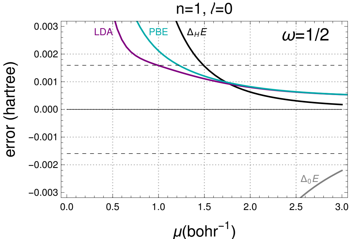
FIG. 4. Errors in the ground state energy estimate for harmonium ( \omega = 1/2 ) using density functional approximations ( \mu -LDA and \mu -PBE). Also shown are the errors of the model energy, \Delta_0 E(\mu) , gray curve, and of the expectation value of the physical Hamiltonian, \Delta_H E(\mu) , black curve.
