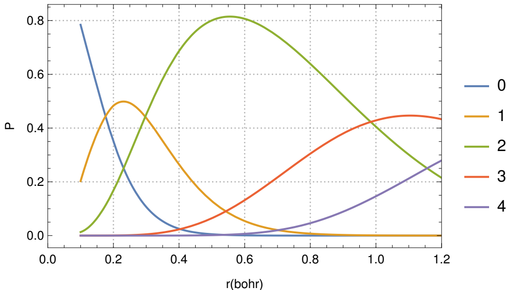
FIG. 3. The probabilities of n = 0, 1, \dots, 4 electrons to be present in a sphere of radius r around the C nucleus in CH 4 .
