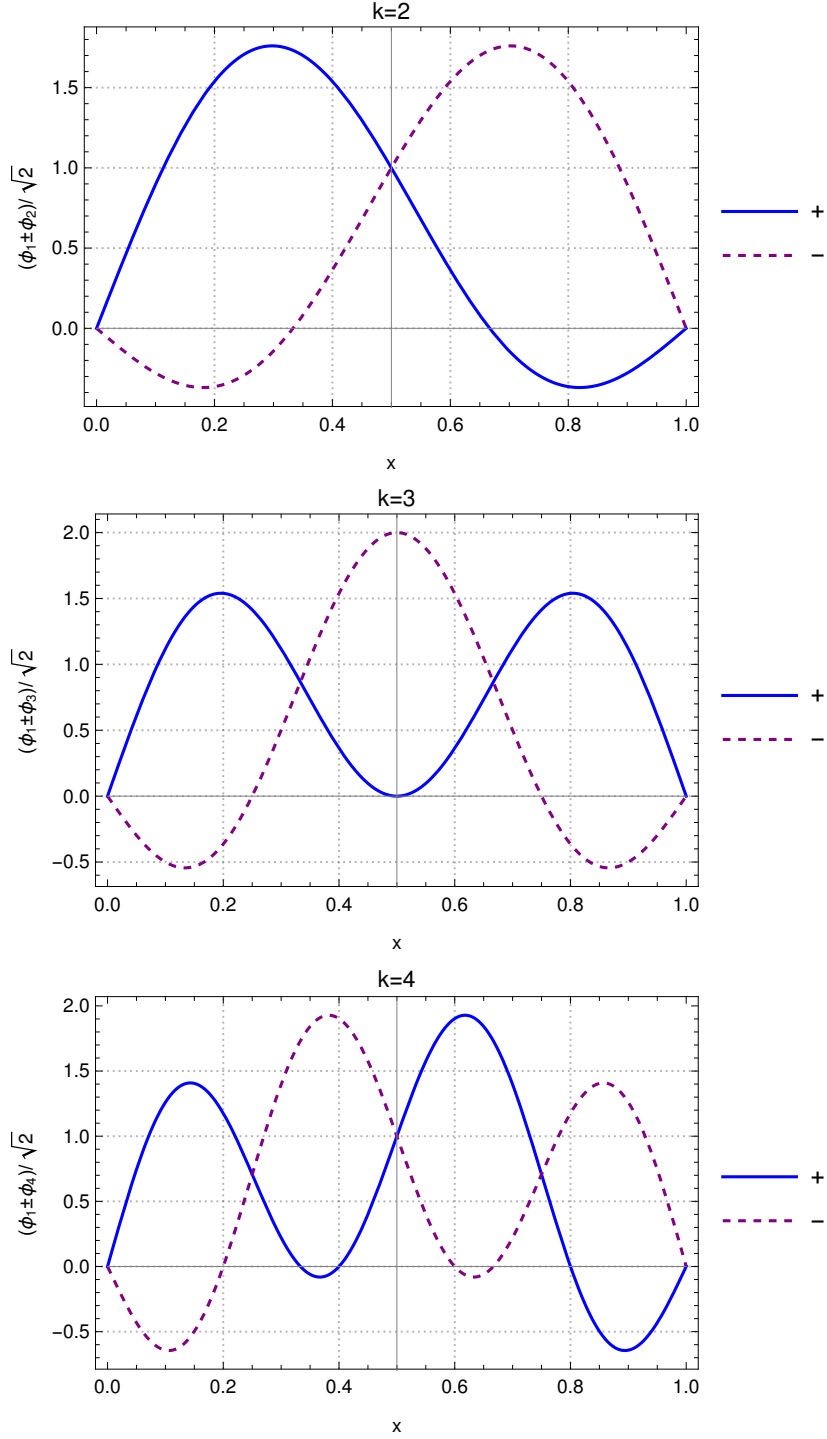
FIG. 2. Localized (equivalent 17 ) orbitals for two independent particles in a one-dimensional box, in a state where the canonical orbitals \phi_1 and \phi_k are occupied; for k = 2 (top panel), k = 3 (middle panel), and k = 4 (bottom panel).
