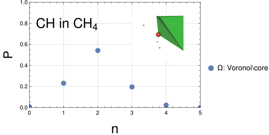
FIG. 4. Probability to find n electrons in the region attributed to the CH bond in \text{CH}_4 . The region is shown in the top right corner of the plot, the (excluded) C core region being also shown, in red.
