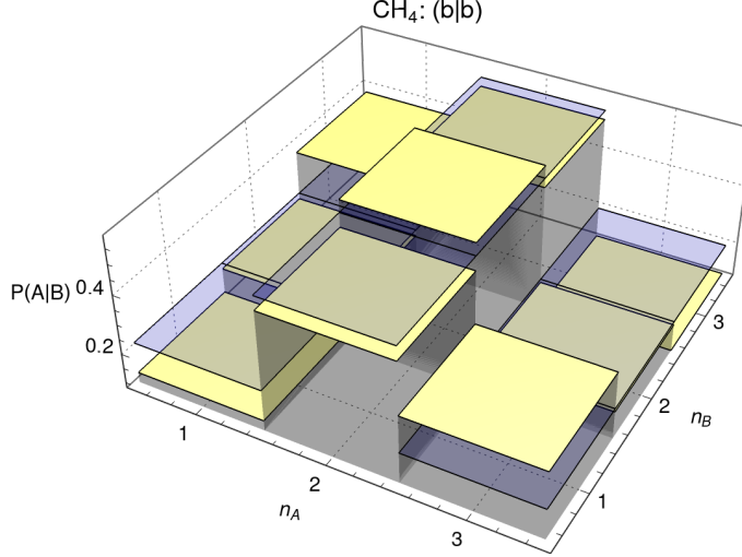
FIG. 9. The conditional probability P_{A|B} of having n_A electrons in region A given that there are n_B electrons in region B , for CH 4 ; A and B correspond to two different CH bond regions. The horizontal semi-transparent blue planes show P_A(n_A) .
