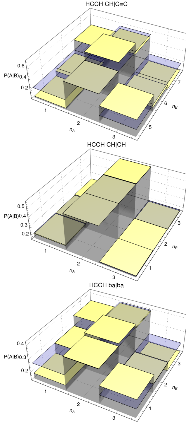
FIG. 10. The conditional probability P_{A|B} of having n_A electrons in region A given that there are n_B electrons in region B , for HCCH (top: A=CH , B=CC , middle A, B are two different CH regions, bottom: A, B are two different banana bonds). The horizontal semi-transparent blue planes show P_A(n_A) .
