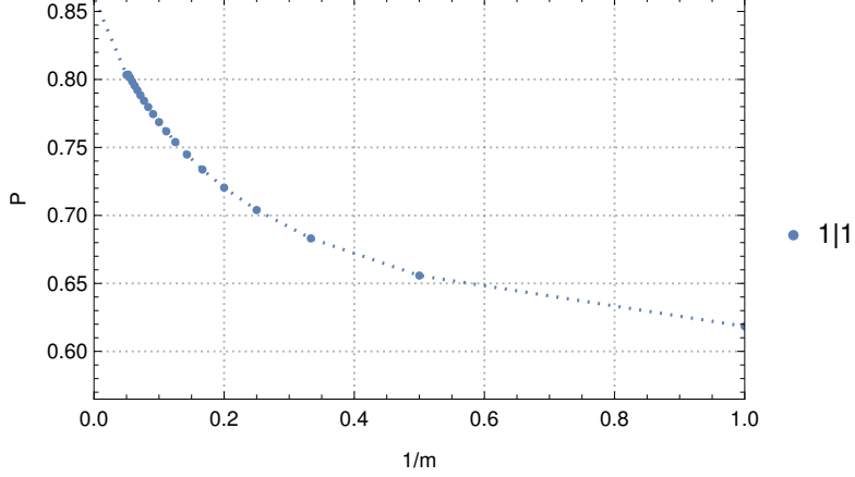
FIG. 17. Probability of having one electron in dominantly in the left half of the box (and another electron dominantly in the right half of the box) as a function of the smoothing (using the smoothstep function S_k , Eq. (B3)). The dotted line is connecting the points to guide the eye.
