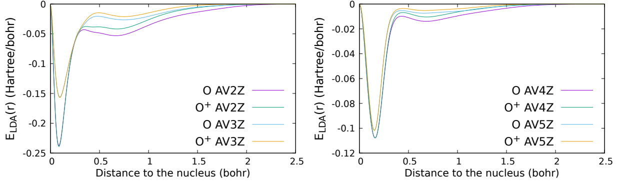
FIG. 7. Behavior of \bar{E}_{\text{LDA}}^{\mathcal{B}}(r) for the AV2Z and AV3Z basis sets (left plot) and AV4Z and AV5Z basis sets (right plot) for the oxygen atom and its first cation.
