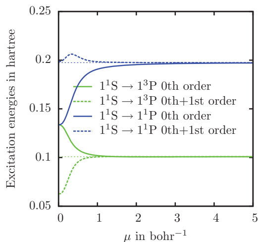
Figure 3. Valence excitation energies of the beryllium atom (in hartree) at zeroth order \Delta\mathcal{E}_k^\mu (plain line) and zeroth + first order \Delta E_k^{\mu,(0+1)} (dashed line), as a function of \mu (in \text{bohr}^{-1} ). The excitation energies of the physical system \Delta E_k are plotted as horizontal dotted lines.
