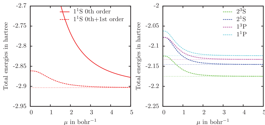
Figure 1. Zeroth + first-order ground- (left) and excited-state (right) total energies E_k^{\mu,(0+1)} (in hartree) of the helium atom as a function of \mu (in \text{bohr}^{-1} ). The zeroth-order energy \mathcal{E}_0^\mu is recalled for the ground state in plain line and the total energies of the physical system E_k are plotted as horizontal dotted lines.
