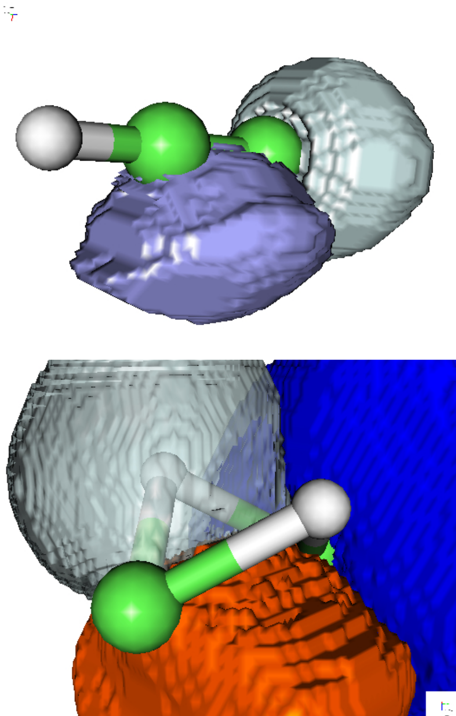
FIG. 3. MPDs in acetylene C_2H_2 , top, and Si_2H_2 , bottom. The MPDs containing the H nuclei are silver-colored; one of the triple banana bond MPDs in C_2H_2 is shown in purple; the lone pair of Si is shown dark blue while the bent Si-Si bond MPD is shown in red.
