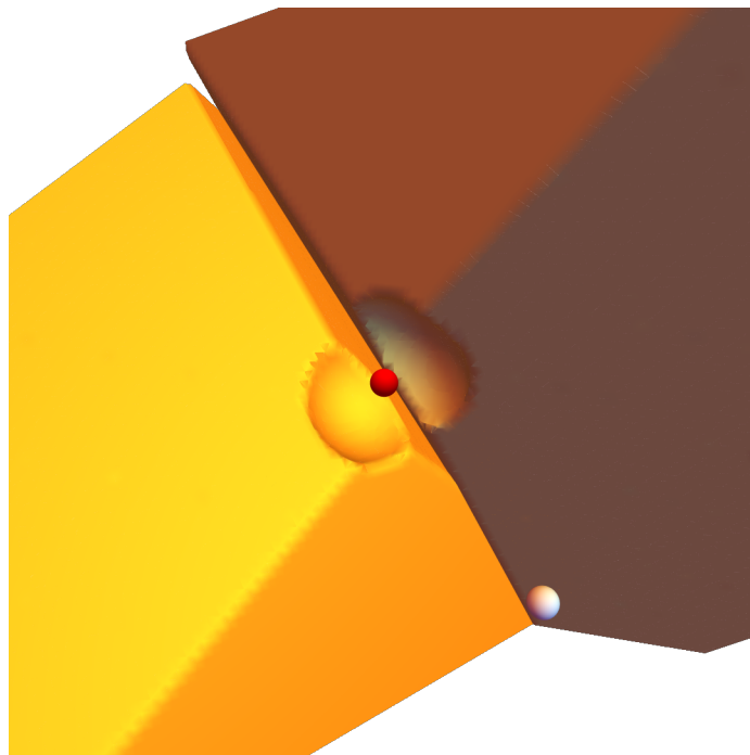
FIG. 2. Spatial domains that maximize the probability for a domain associated to the OH bond electron pair (orange), or the O lone pair (brown), by excluding a region associated to the O core, and by defining Voronoi cells with moving centers. The positions of the nuclei are indicated by small spheres (red: O, white: one of the H atoms, the other being hidden behind the orange surface).
