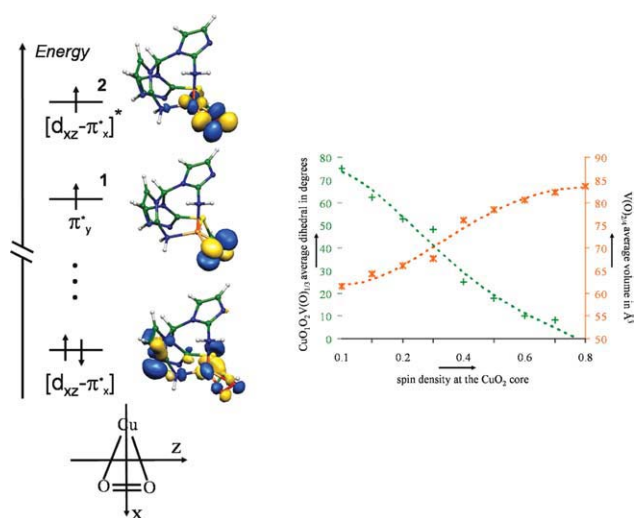
Figure 3. Left: MOs resulting from the interaction between the dioxygen \pi_x^* and \pi_y^* molecular orbitals and the copper d_{xz} orbital for the case of the [(\text{Mim}^{\text{N2S}})\text{Cu}(\text{O}_2)]^+ complex. Right: evolution of the average \text{CuO}_1\text{O}_2\text{V}(\text{O})_{1/3} dihedral angles as a function of the spin density at the \text{CuO}_2 core on progressive injection of one electron (constrained DFT computations) at a frozen geometry.
